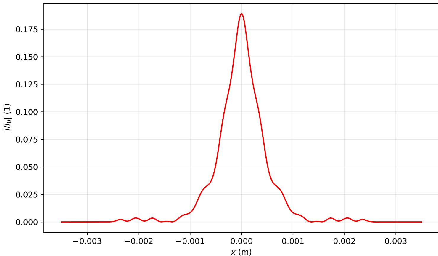
Intensity profile I(x, y = 0, z = 2.707)/I_0 , P_{in}=5.0P_{cr} , artificial time
